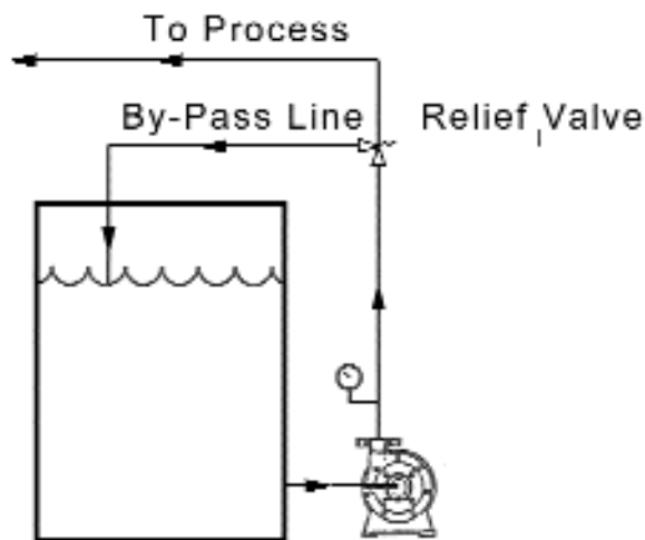
Figure 2: By-pass Configuration
