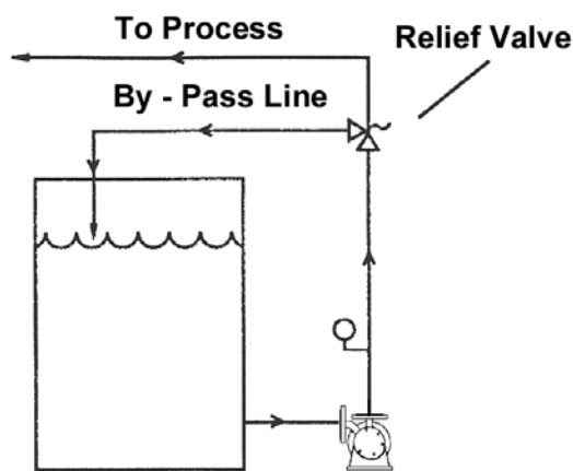
Figure 2: By-pass Configuration
